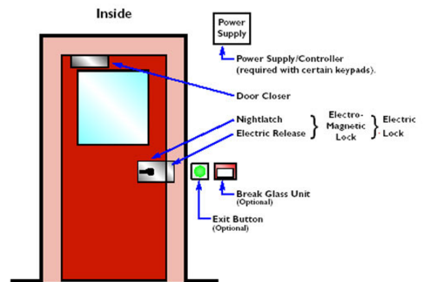
Model : Break Glass Fire Emergency Exit Release
